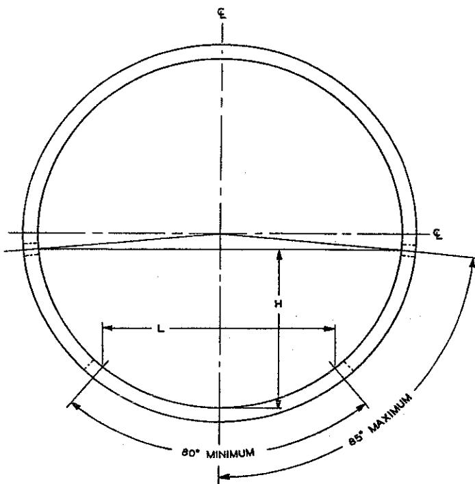
FIG. 1 Requirements for Perforations
